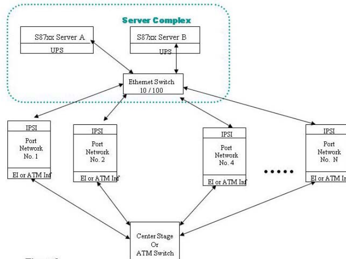
Figure 3 S87xx Sever Based System “Duplex” or Standard Reliability
